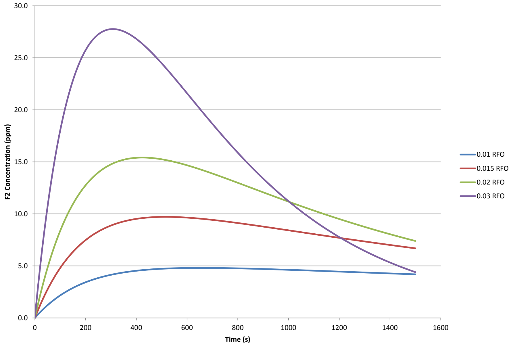
F2 Concentration with various RFO sizes (assuming perfect mixing)
