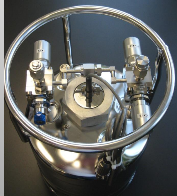
Proprietary 4-valve config. Optimized for Low V.P. precursors Dead-leg free design utilizing CDS Labs surface mount manifolds
